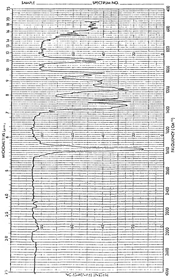
Figure 29 - Infrared Spectrum of \text{CF}_2=\text{CHCF}_2\text{CF}=\text{CF}_2
